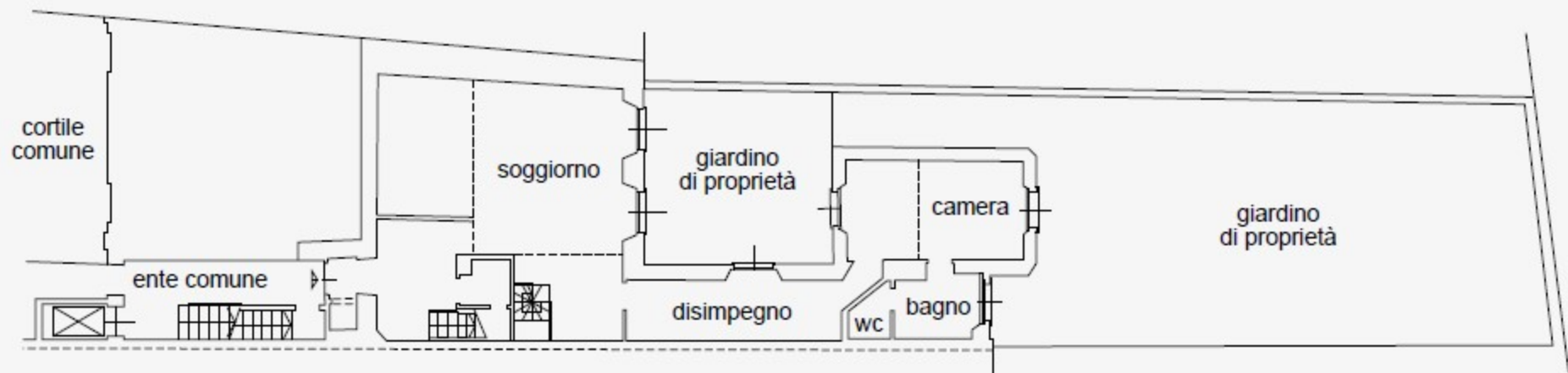
PIANO TERRA
